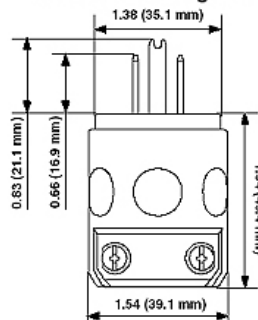
Dimensional Diagram
